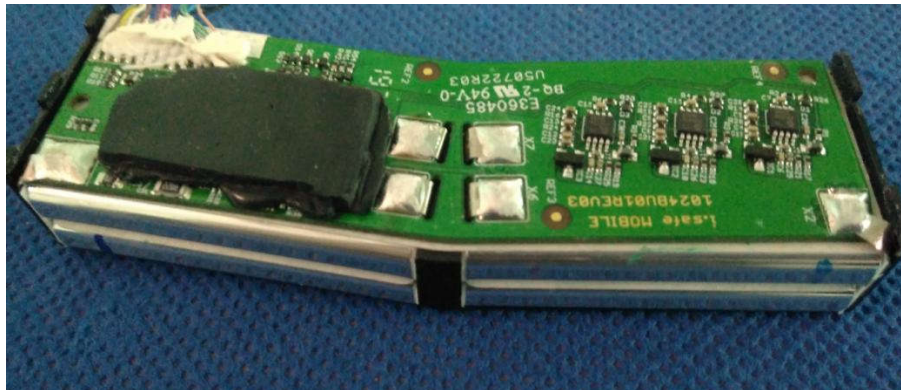
电池内部结构 Battery internal structure
