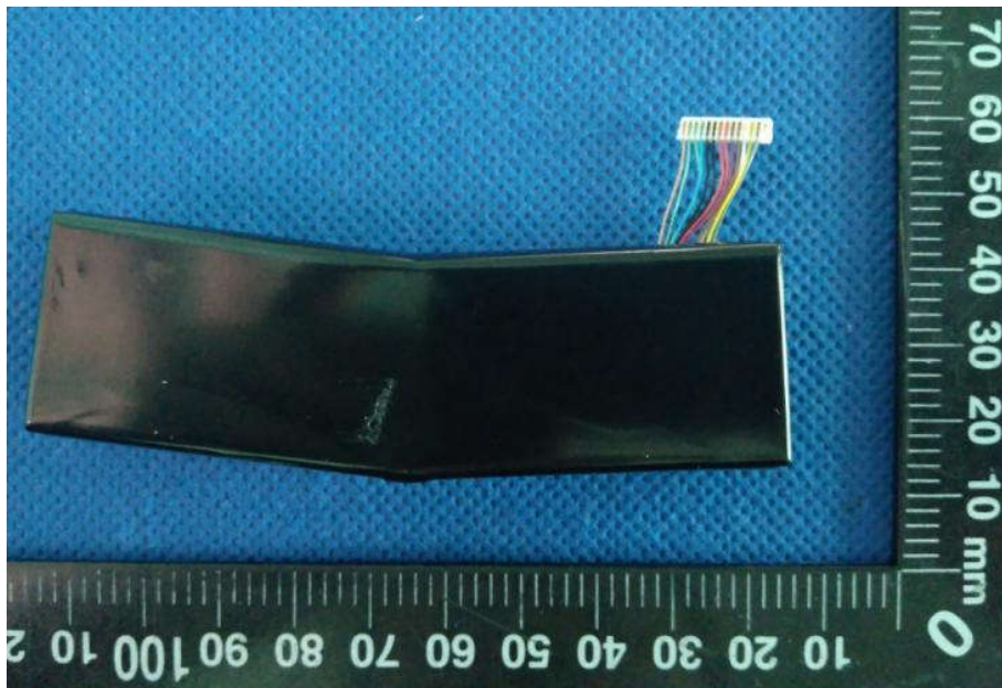
电池组外观 2 View of the battery 2
